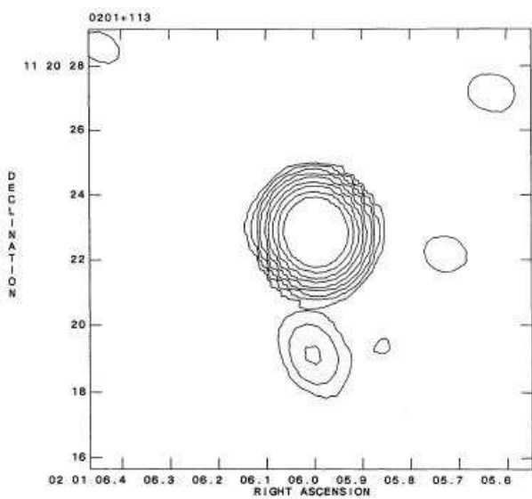
Fig. 1. Contour plot of 0201+113 at 18 cm with a resolution (FWHM) of 1''.29 \times 1''.16 at position angle 18^\circ . The contours are the rms noise (0.18 mJy/beam) times -3, 3, 6, 12, 24, 50, 100, 200, 400, 800
