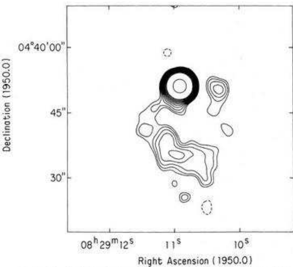
FIG. 1g.—0829+046, 50,000 wavelength taper. Peak flux density: 639 mJy beam -1 . Lowest contour: 0.2%.
