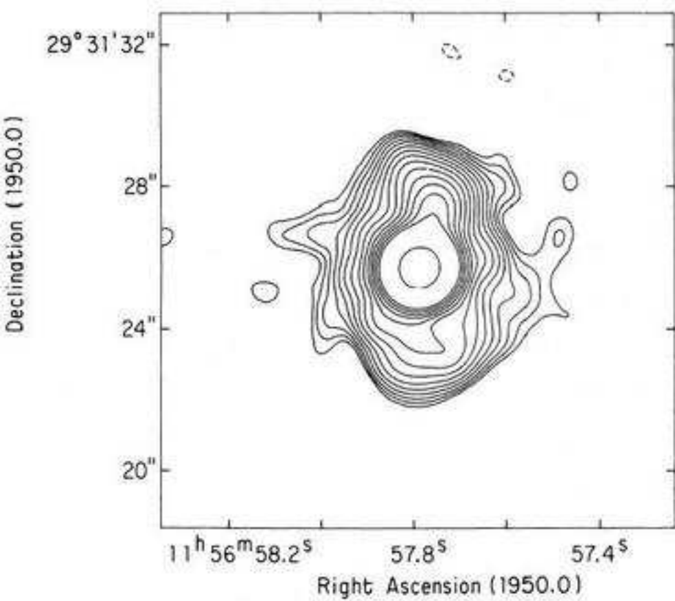
FIG. 1k.—1156+295, full resolution. Peak flux density: 1307 \text{ mJy beam}^{-1} . Lowest contour: 0.07%.
