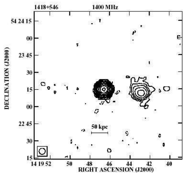
Fig.18. 1418+546, VLA B configuration, 1.40 GHz (from FIRST, Becker et al. 1995). The restoring beam is 5.4 \times 5.4 arc-sec. The peak flux density is 566 mJy/beam and the rms noise on the image is 0.15 mJy/beam
