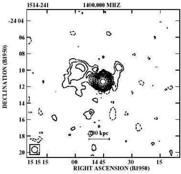
Fig. 23. 1514—241; VLA D configuration, 1.40 GHz (from NVSS, Condon et al. 1998). The restoring beam is 45.0 \times 45.0 arcsec. The peak flux density is 1993 mJy/beam and the rms noise on the image is 0.40 mJy/beam
