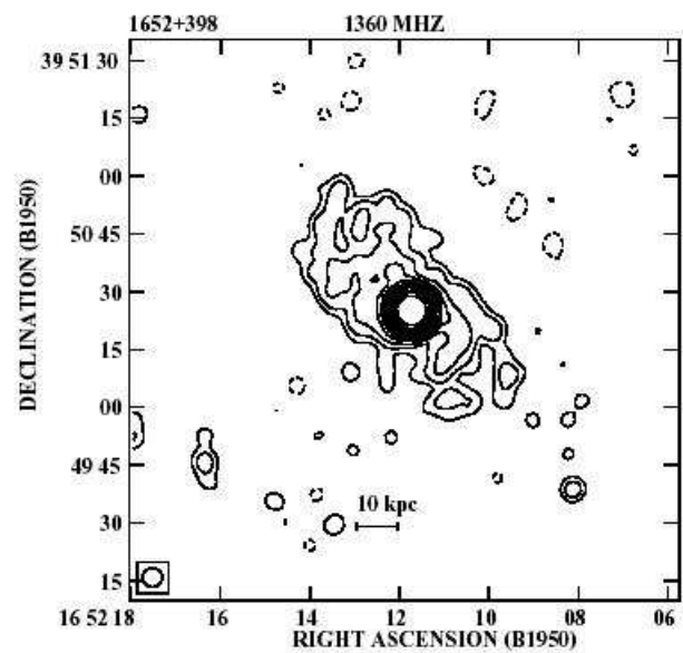
Fig. 24. 1652+398, VLA B configuration, 1.36 GHz. The restoring beam is 3.5 \times 3.0 arcsec in PA -84^\circ . The peak flux density is 1383 mJy/beam and the rms noise on the image is 0.13 mJy/beam
