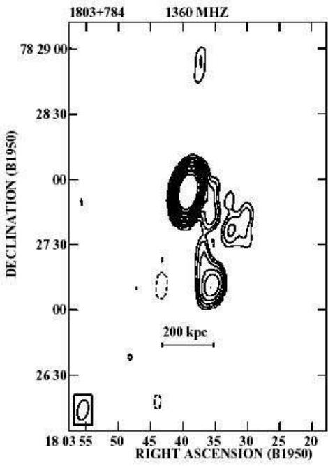
Fig. 26. 1803+784, VLA B configuration, 1.36 GHz. The restoring beam is 9.3 \times 4.9 arcsec in PA -11^\circ . The peak flux density is 1761 mJy/beam and the rms noise on the image is 0.07 mJy/beam
