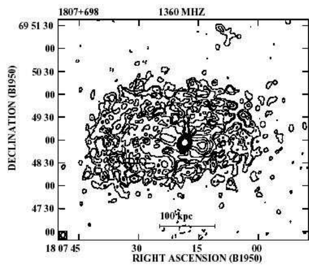
Fig. 27. 1807+698, VLA A+B+D configuration, 1.36 GHz. The restoring beam is 7.0 \times 5.5 arcsec in PA -22^\circ . The peak flux density is 1284 mJy/beam and the rms noise on the image is 0.10 mJy/beam
