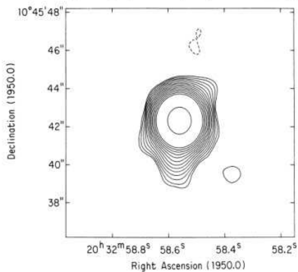
FIG. 1F+2032+107, full resolution. Peak flux density: 764 mJy beam -1 . Lowest contour: 0.1%.
