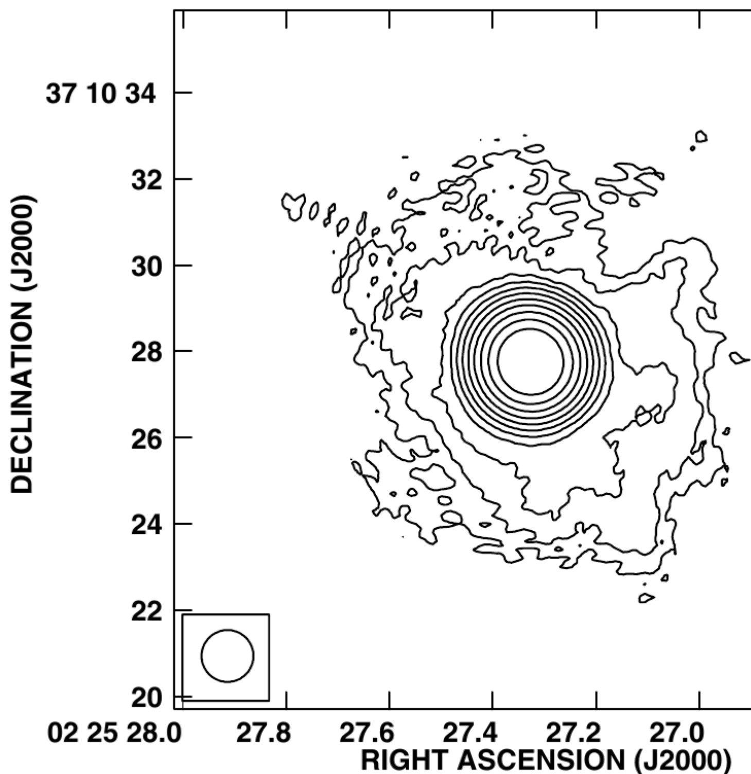
Fig. 2. Image of 0222+36 at 5 GHz, VLA in “A+B” configuration. Contours are traced at (1, 2, 4, 8, ...) times the 3\sigma noise. The lowest contour is 69 \mu\text{Jy/beam} , the peak is 209 \text{ mJy/beam} , and the beam is circular with a HPBW of 1.2'' .
