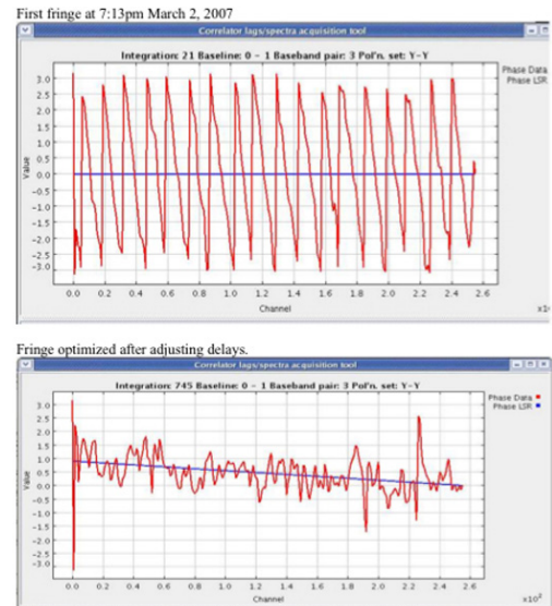
The successful “first fringes” observations of Saturn at 104 GHz. The planet was tracked for more than an hour by the ALMA system.
