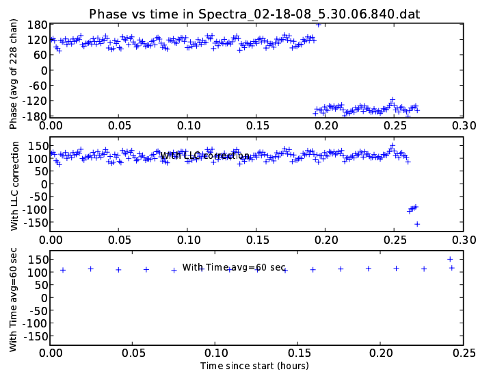
Fig. 5.— 0359 Xref=VaPax, Yref=VaPay, Zref=VaPaz, vaAntenna.zPosition.value = 4,ae-cAntenna.zPosition.value = 4
