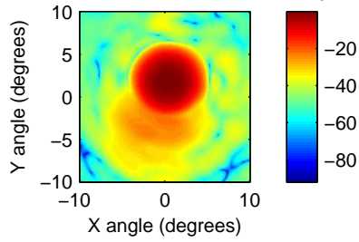
2007_Scan_13_Beam_1_FF.csv: amp
