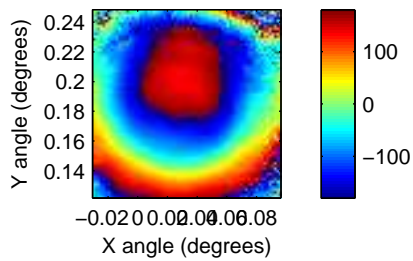
2007_Scan_13_Beam_1_NF.csv: phase
