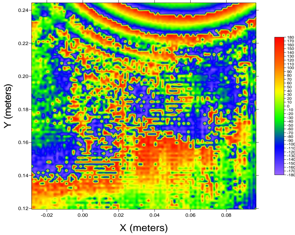
Near-field phase of NRAO FE2 band3 109.NSI
