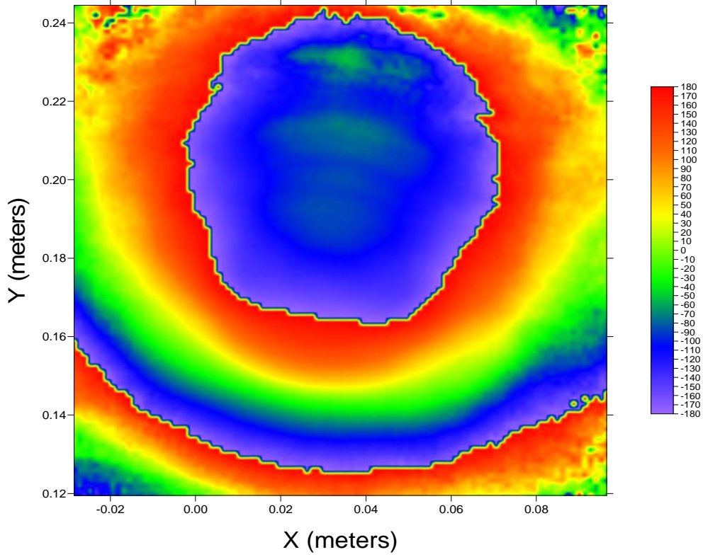
Near-field phase of NRAO FE2 band3 100.NSI
