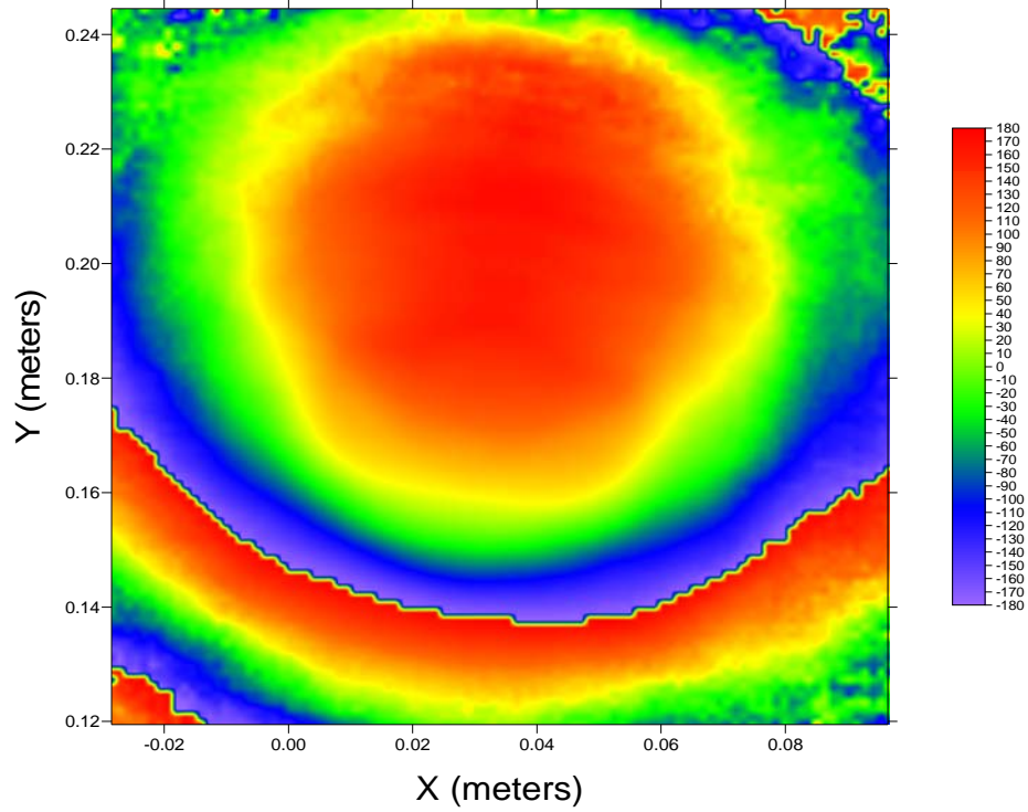
Near-field phase of NRAO FE2 band3 100.NSI
