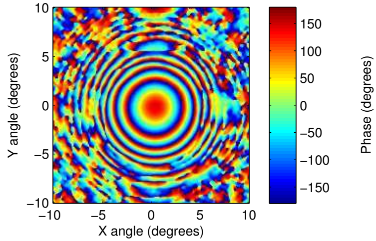
NRAO_FE1_band9_2007-11_Scan_77_FF.csv: phase
