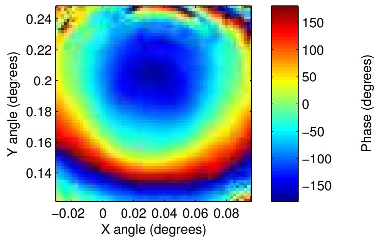
2007_Scan_17_NF.csv: phase
