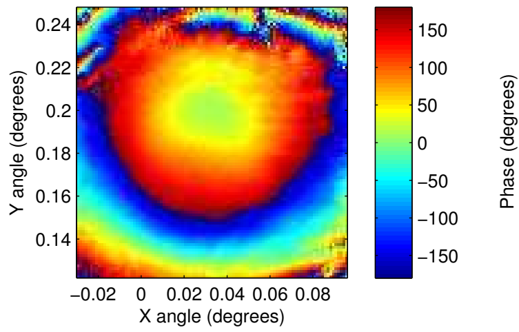
2008_Scan_8_NF.csv: phase
