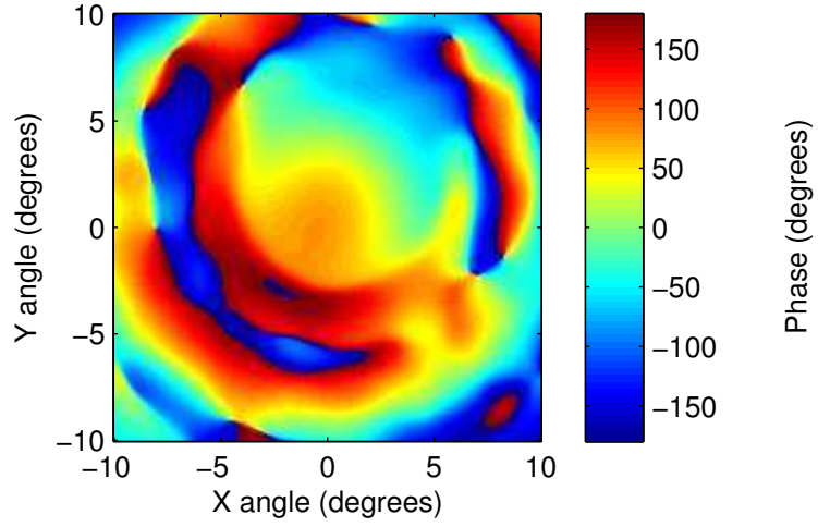
2007_Scan_22_FF.csv: phase
