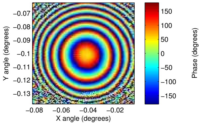
NRAO_FE1_band9_2007-11_Scan_77_NF.csv: phase
