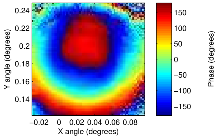
2007_Scan_13_NF.csv: phase
