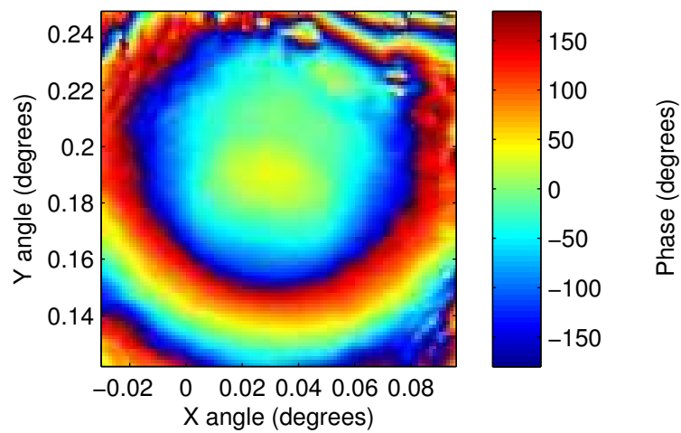
2008_Scan_17_NF.csv: phase
