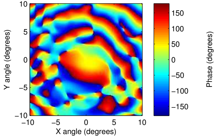
2008_Scan_20_FF.csv: phase
