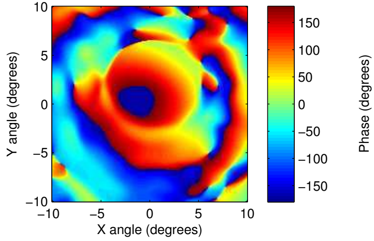
2007_Scan_19_FF.csv: phase
