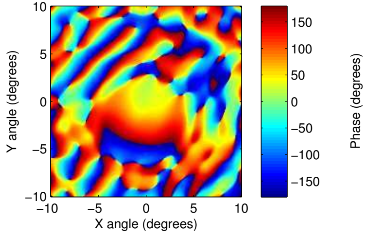
2008_Scan_22_FF.csv: phase
