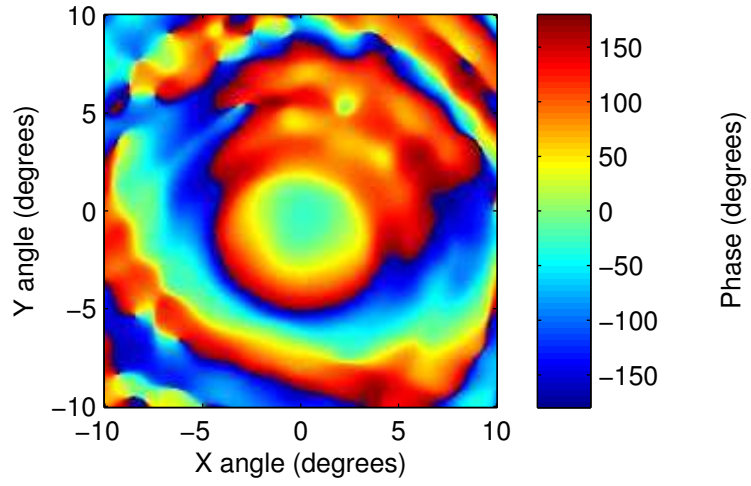
2008_Scan_4_FF.csv: phase
