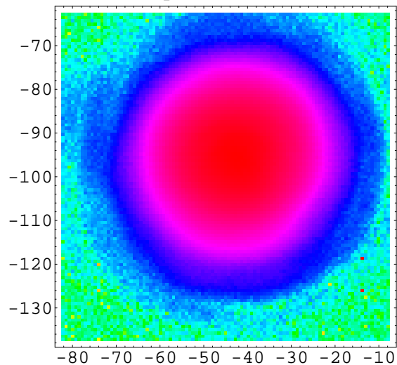
Near-field amplitude, Band 9, Scan 77
