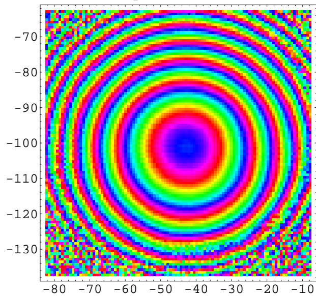
Near-field phase, Band 9, Scan 77
