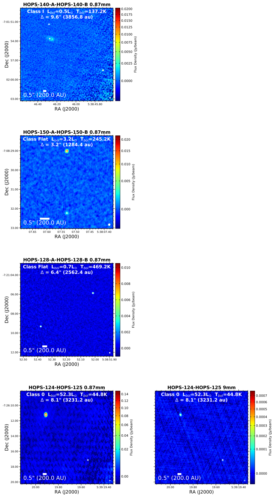
Figure 68. Orion Wide Multiple Images
