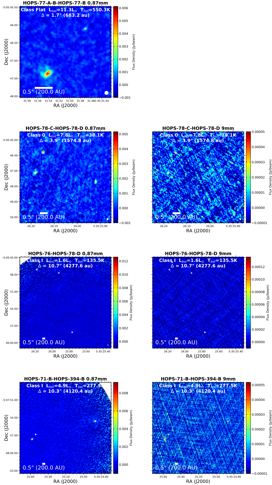
Figure 61. Orion Wide Multiple Images
