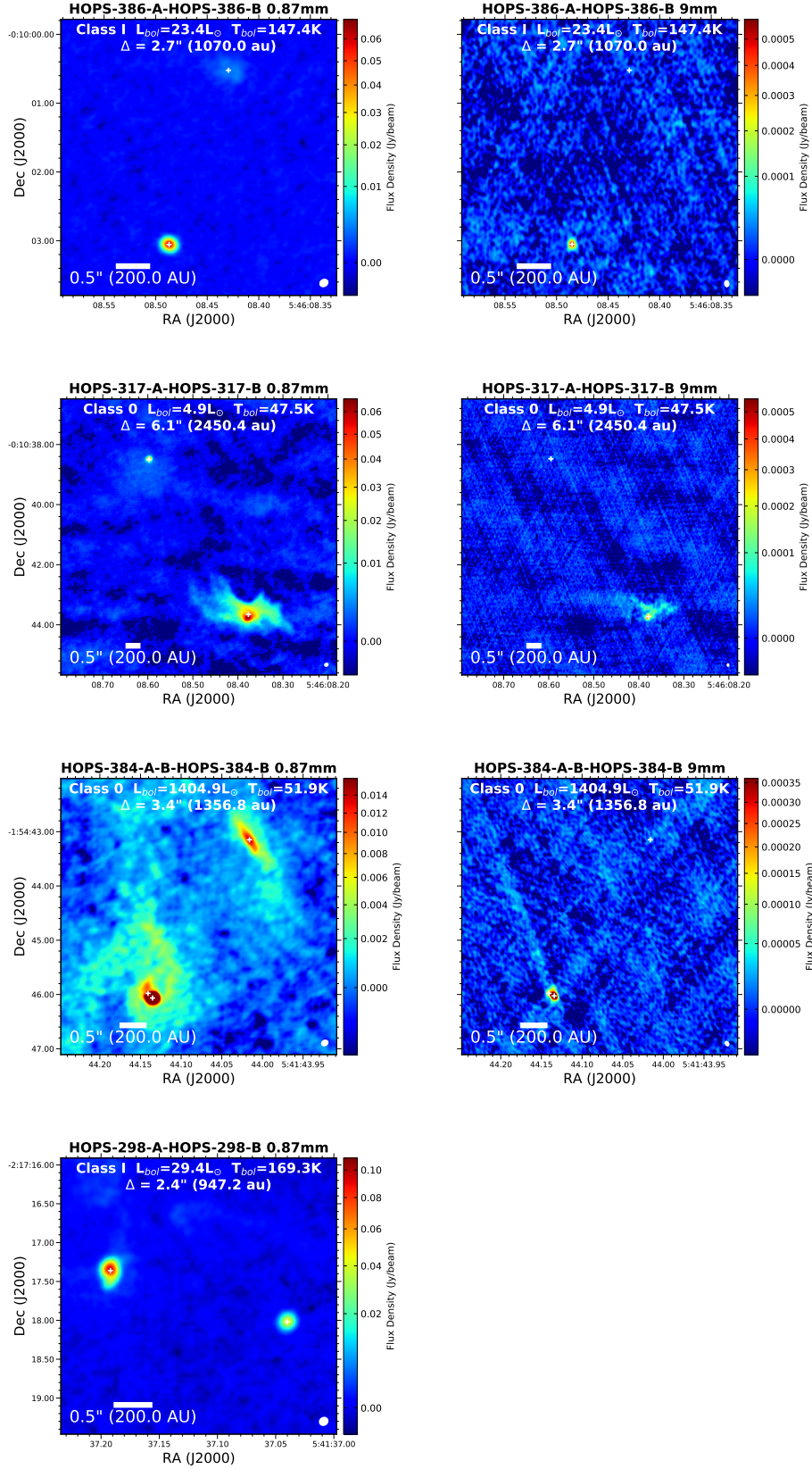
Figure 59. Orion Wide Multiple Images
