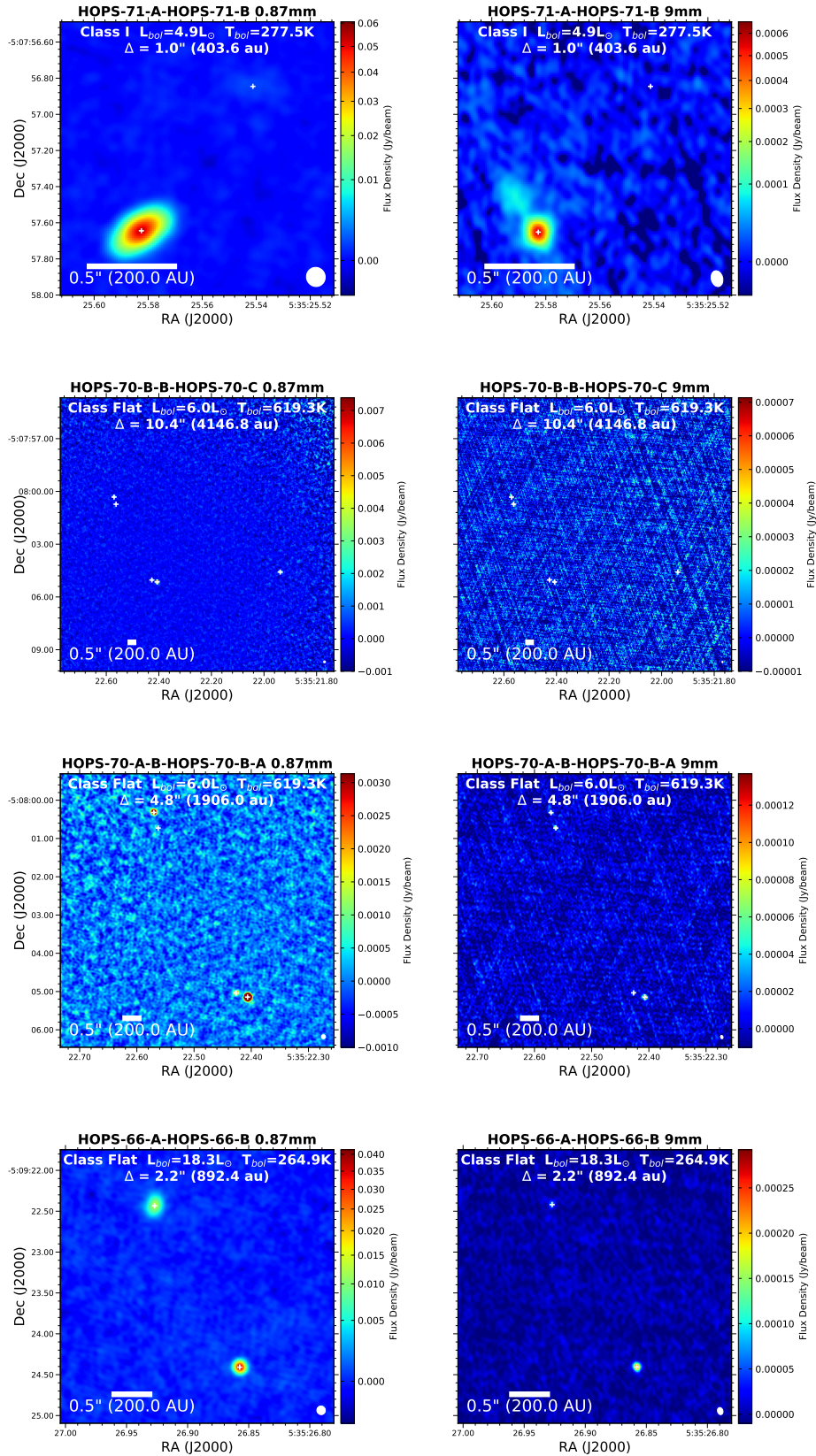
Figure 62. Orion Wide Multiple Images
