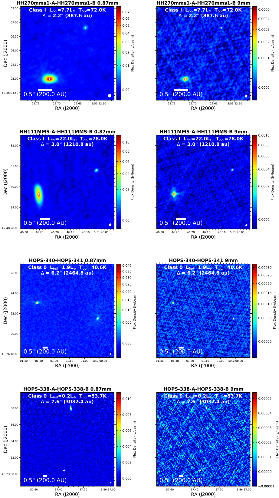
Figure 55. Orion Wide Multiple Images
