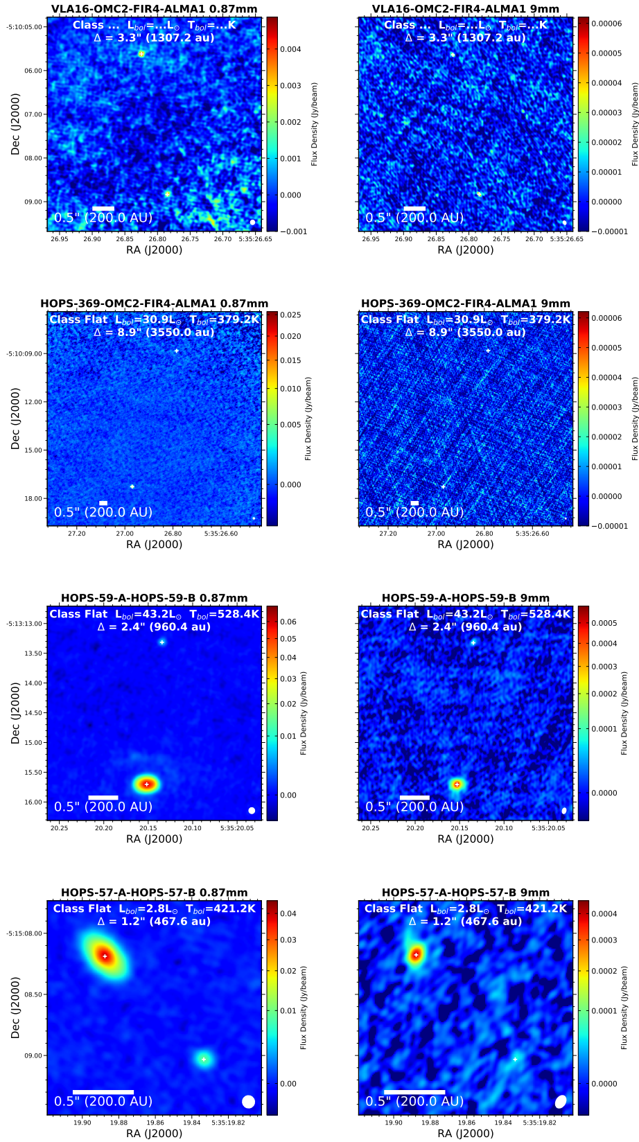
Figure 64. Orion Wide Multiple Images
