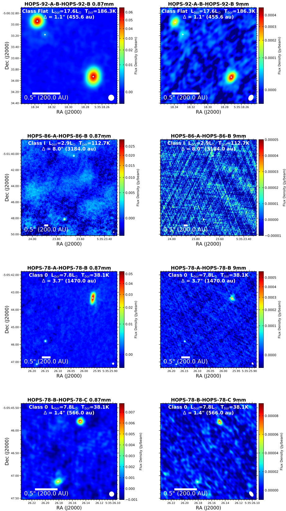
Figure 60. Orion Wide Multiple Images
