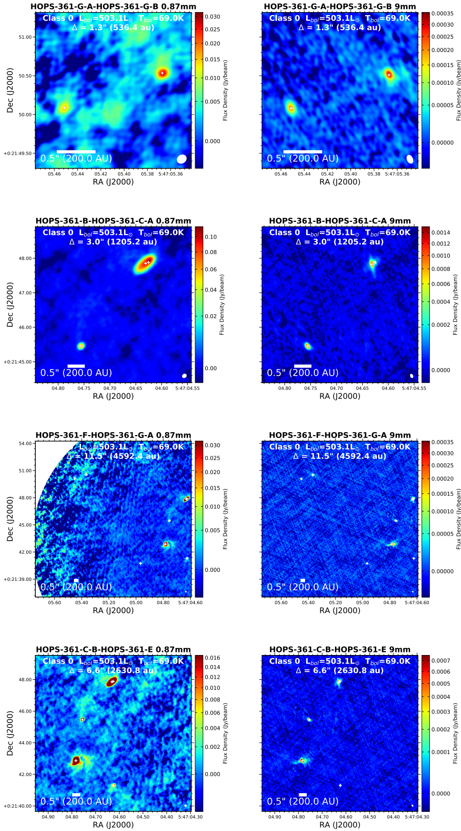
Figure 56. Orion Wide Multiple Images
