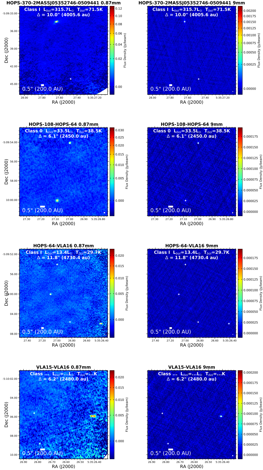
Figure 63. Orion Wide Multiple Images
