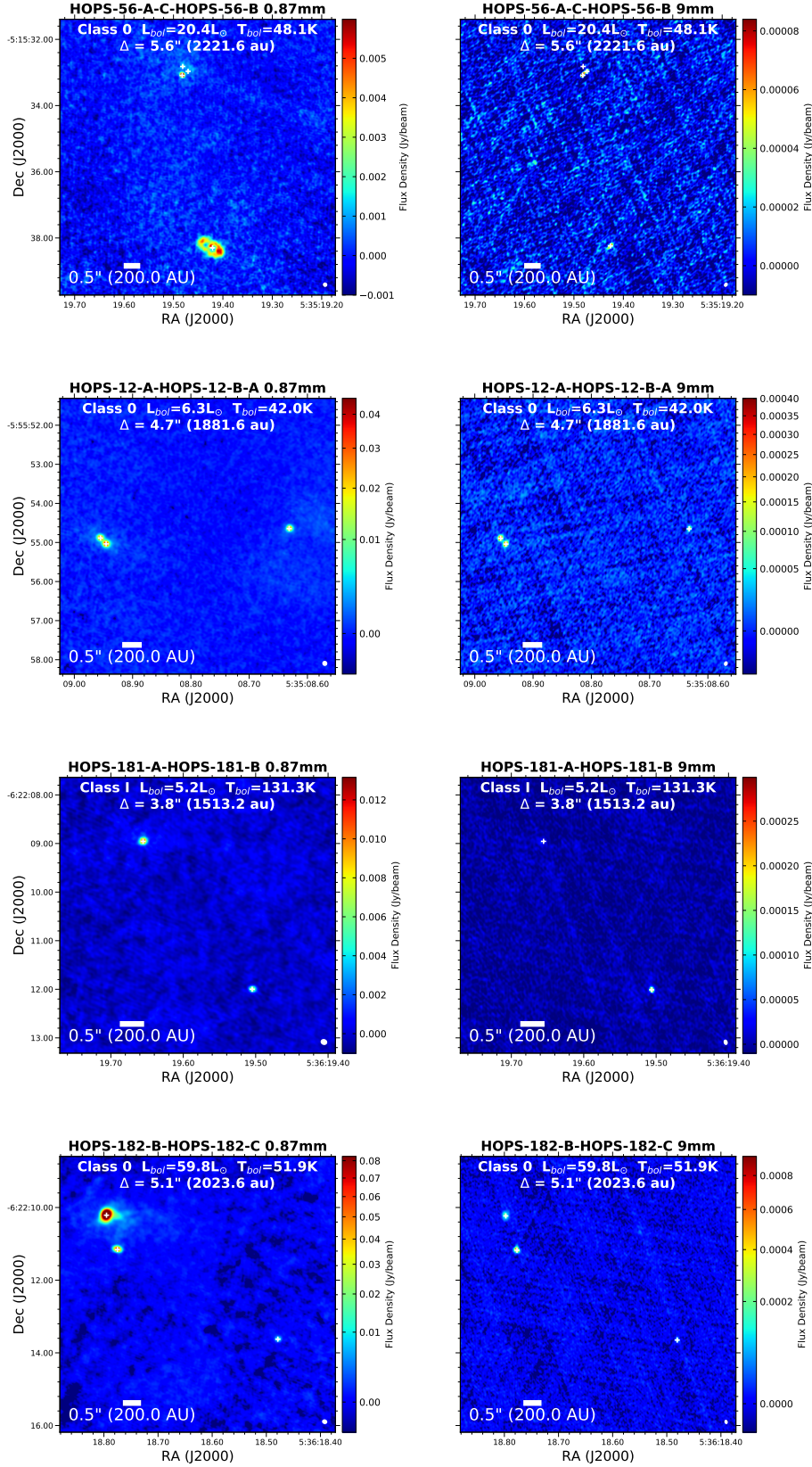
Figure 65. Orion Wide Multiple Images
