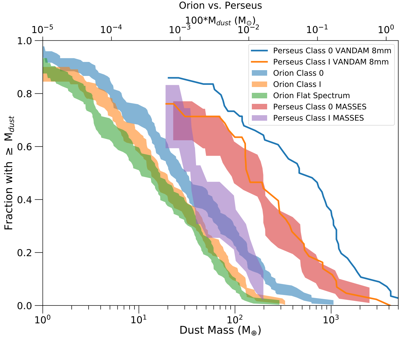
Figure 70. Cumulative distributions of dust disk masses within the full Orion sample relative to the protostellar dust disk mass measurements in Perseus from both VANDAM (Tychoniec et al. 2018) and MASSES (Andersen et al. 2019). The mass distributions from Tychoniec et al. (2018) are drawn as lines in this plot for clarity. This comparison enables us to explore differences that might be due to the wavelengths observed. The values from Andersen et al. (MASSES; 2019) indicate systematically lower masses than those in Tychoniec et al. (VANDAM; 2018), but are still not consistent with the mass distributions of the Orion sample.
