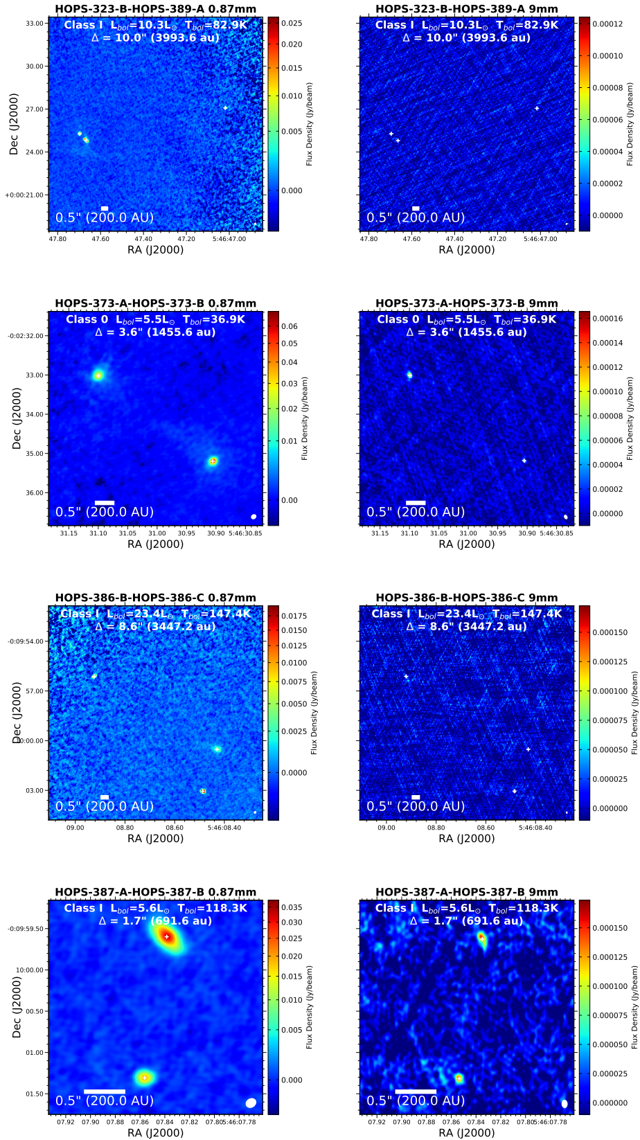
Figure 58. Orion Wide Multiple Images
