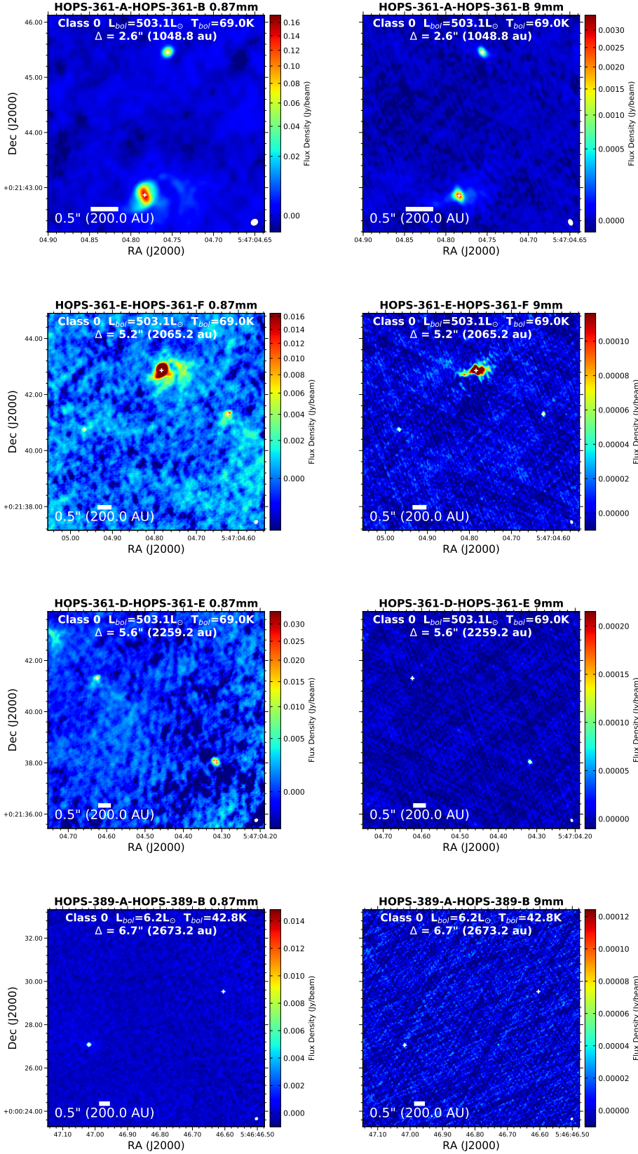
Figure 57. Orion Wide Multiple Images
