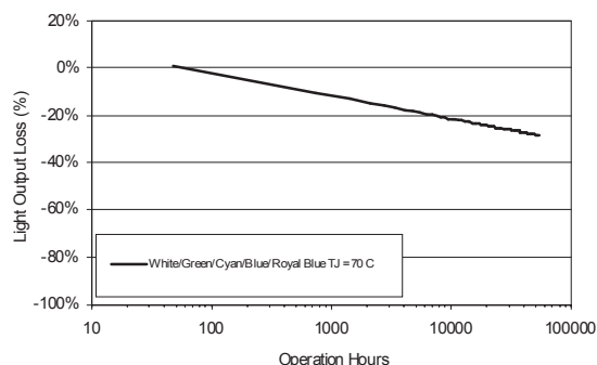
Figure 14. Light Output vs. Time for White, Green, Cyan, Blue and Royal Blue at I_f 350mA, Relative Humidity less than 25%.
