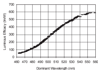
Figure 5. Luminous Efficacy vs. Dominant Wavelength for InGaN Material.
