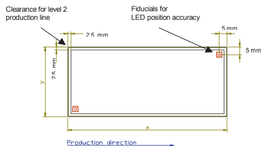
Figure 41. Board Clearance and Fiducials.
