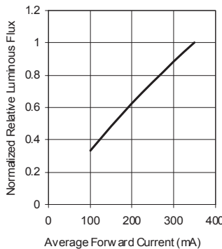
Figure 31. Relative Luminous Flux vs. Forward Current for Green, Cyan, Blue, Royal Blue, and White.
