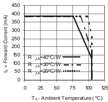
Figure 33. Maximum Forward Current vs. Ambient Temperature. Derating based on T_{JMAX} = 120^{\circ}\text{C} for Red, Red-Orange and Amber.
