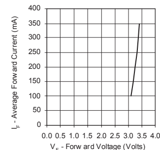
Figure 28. Forward Current vs. Forward Voltage for Green, Cyan, Blue, Royal Blue and White.
