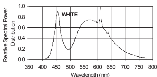
Figure 10. Relative Intensity vs. Wavelength for White.
