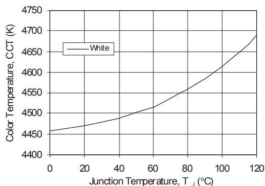
Figure 12. Color Temperature Shift.
