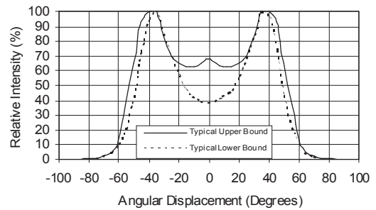
Figure 19. Representative Spatial Radiation Pattern for Red, Amber, Green, Cyan, Blue and Royal Blue.
