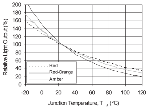
Figure 16. Temporary AlInGaP Light Output Loss (typical performance).
