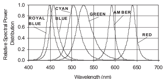
Figure 9. Relative Intensity vs. Wavelength.
