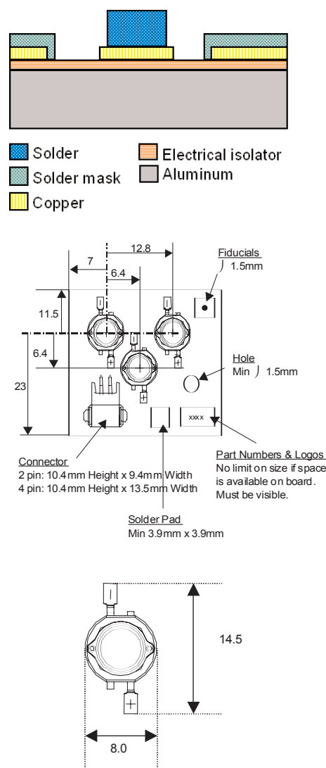
Figure 39. Details of Aluminum-Core PCB.
