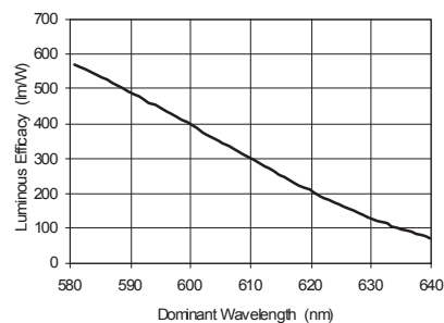
Figure 6. Luminous Efficacy vs. Dominant Wavelength for AlInGaP Material.
