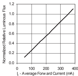
Figure 30. Relative Luminous Flux vs. Forward Current for Red, Red-Orange and Amber.
