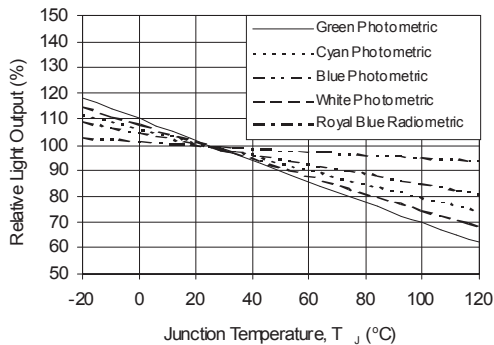
Figure 17. Temporary InGaN Light Output Loss (typical performance).
