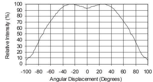
Figure 20. Representative Spatial Radiation Pattern for Red, Red-Orange and Amber.
