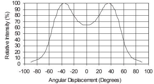
Figure 18. Representative Spatial Radiation Pattern for White.
