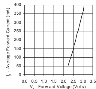
Figure 27. Forward Current vs. Forward Voltage for Red, Red-Orange and Amber.
