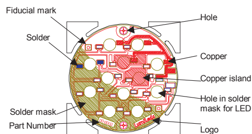
Figure 42. Board Design Example.
