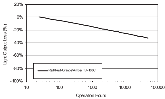
Figure 15. Light Output vs. Time for Amber, Red-Orange and Red at 385mA.
